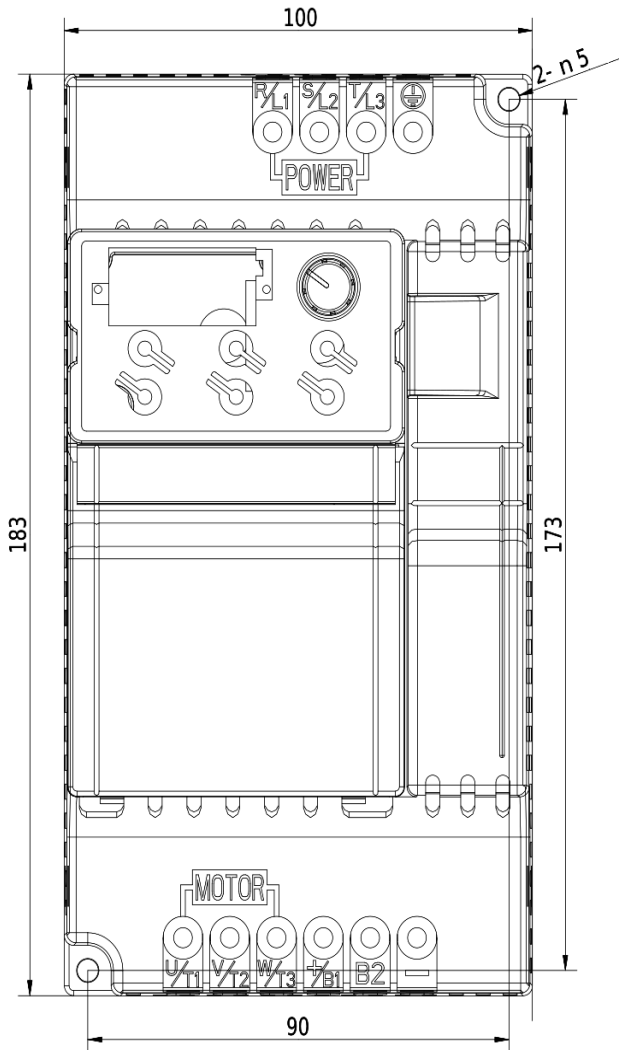
Dimensional drawing V800 - 5,5kW 4T0055
