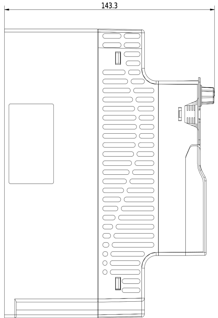
Dimensional drawing V800 - 5,5kW 4T0055
